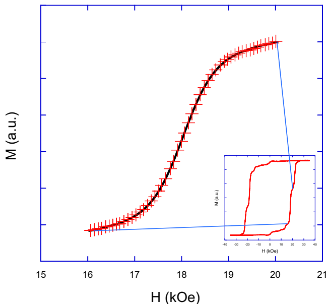
Fig. 3: (Colour on-line) Detail of the N = 4 step with fit. The data was taken at 2.0 K and with no pressure applied. The inset shows the full hysteresis loop from which the detail was taken.
