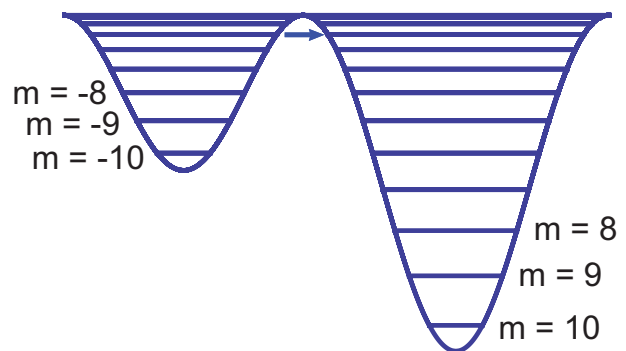
Fig. 1: (Colour on-line) Double-well potential diagram illustrating the energy levels for an S = 10 system. A magnetic field tilts the potential. When the field brings levels in opposite wells into alignment, the spins reverse via a process of resonant tunneling. At temperatures above \sim 0.5 K, this process is thermally assisted and tunneling occurs between levels near the top of the barrier, as indicated by the arrow.
